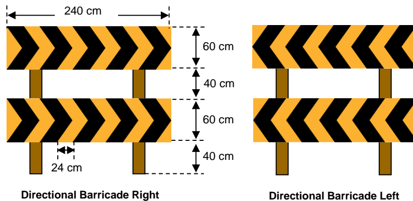
Figure 3-3: Directional Barricades
