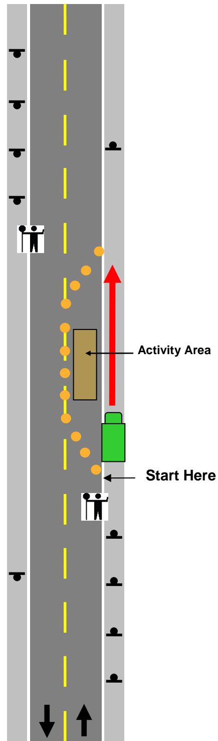
Figure 4-4: Lane Closure Setup (Two Lane Roads)
